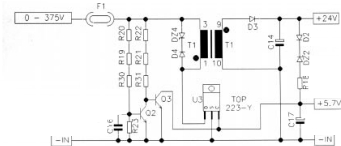
Fig. 4. Auxiliary power supply in line Modules.
